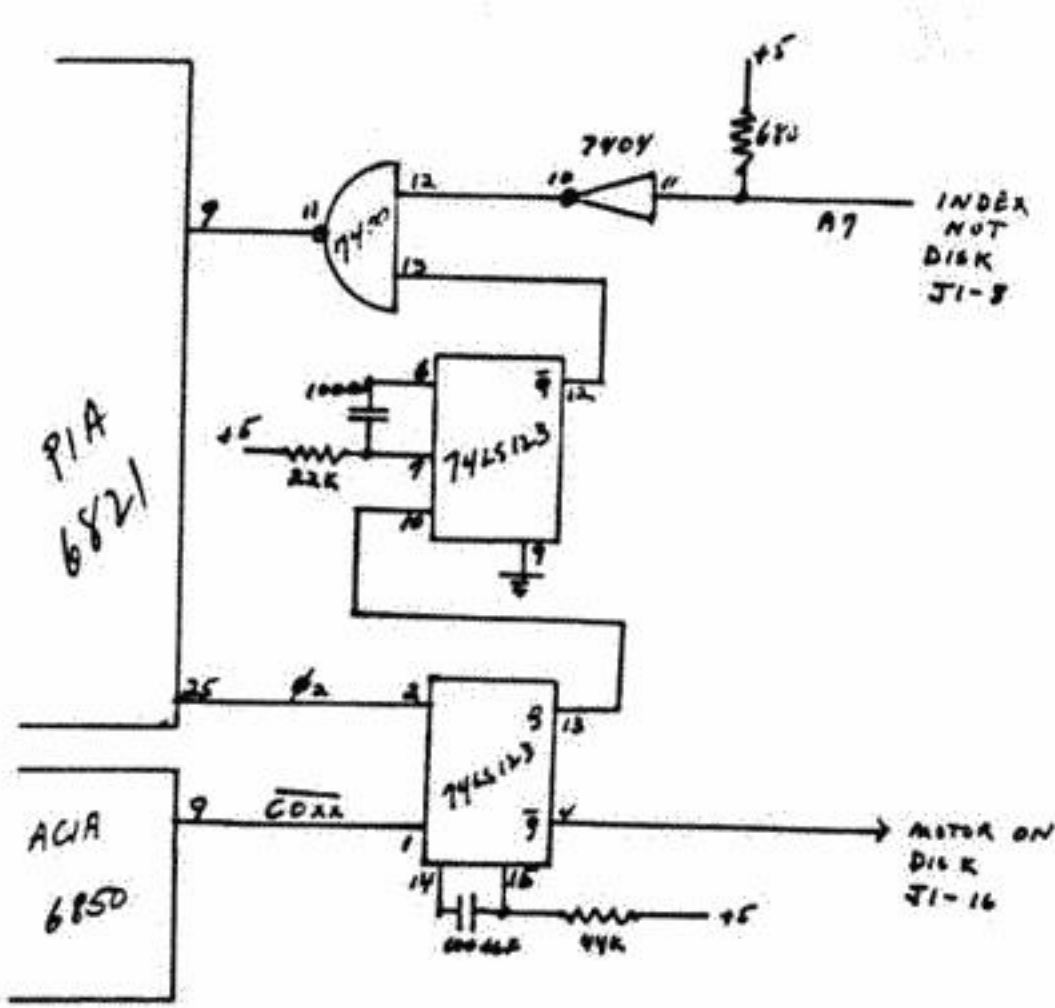
MOTOR CONTROL FIGURE #5
