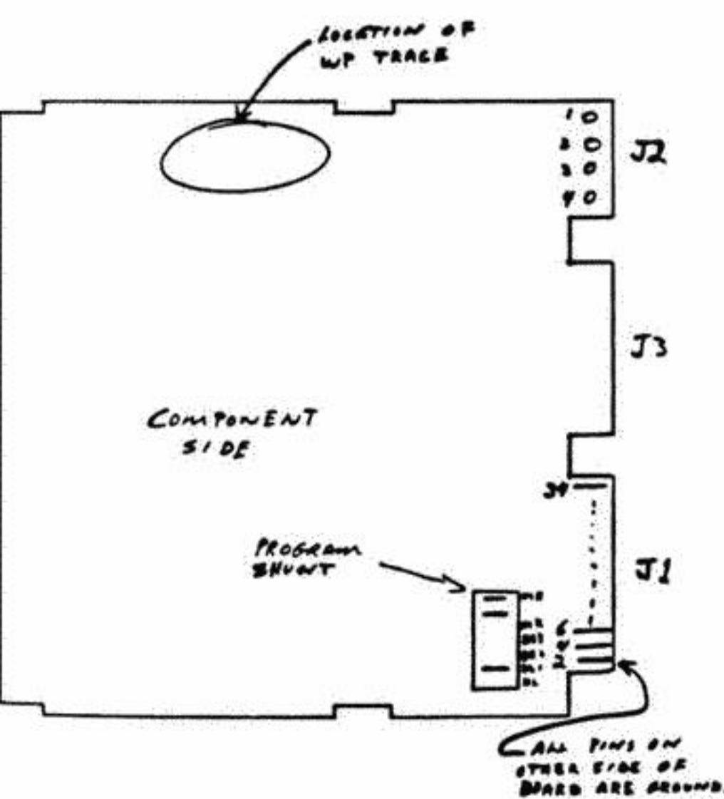
DRIVE PRINTED CIRCUIT BOARD
